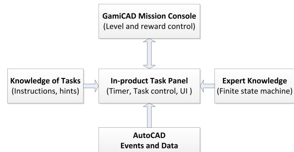
Figure 2. GamiCAD Architecture.
