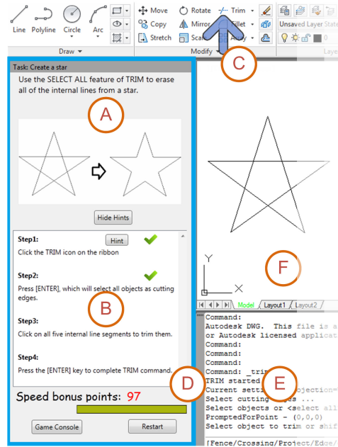
Figure 7. Task panel for SkillBuilder (A) Task description; (B) Step-by-step instructions; (C) UI element visual aid; (D) Speed bonus; (E) AutoCAD command line; (F) Drawing area.
