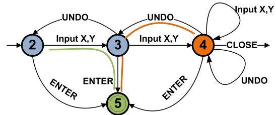
Figure 4. Error recovery. User currently in state 4. Correct flow is green line connecting states 2→3→5. Orange line shows the error recovery path 4→3→5.
