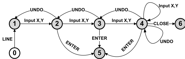
Figure 3. FSMs for LINE command.
